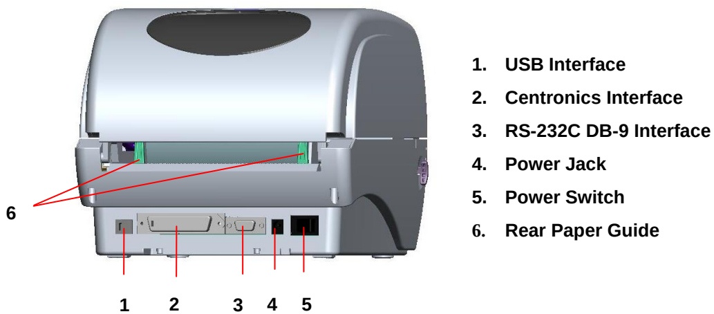
Fig. 2 Rear view
