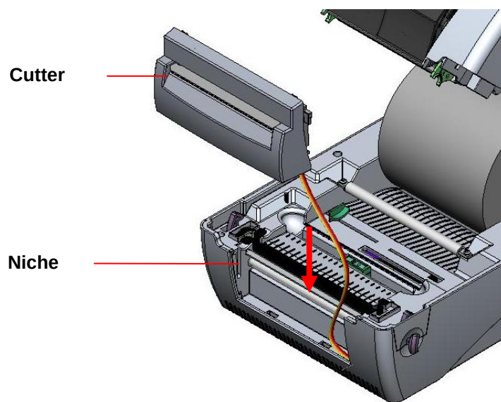
Fig. 26 Cutter module installation
