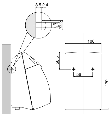
Hooks for wall mounting
