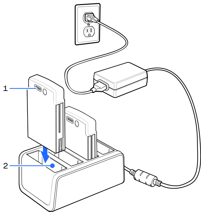
Figure 37 4-Slot PowerPack Battery Charger
