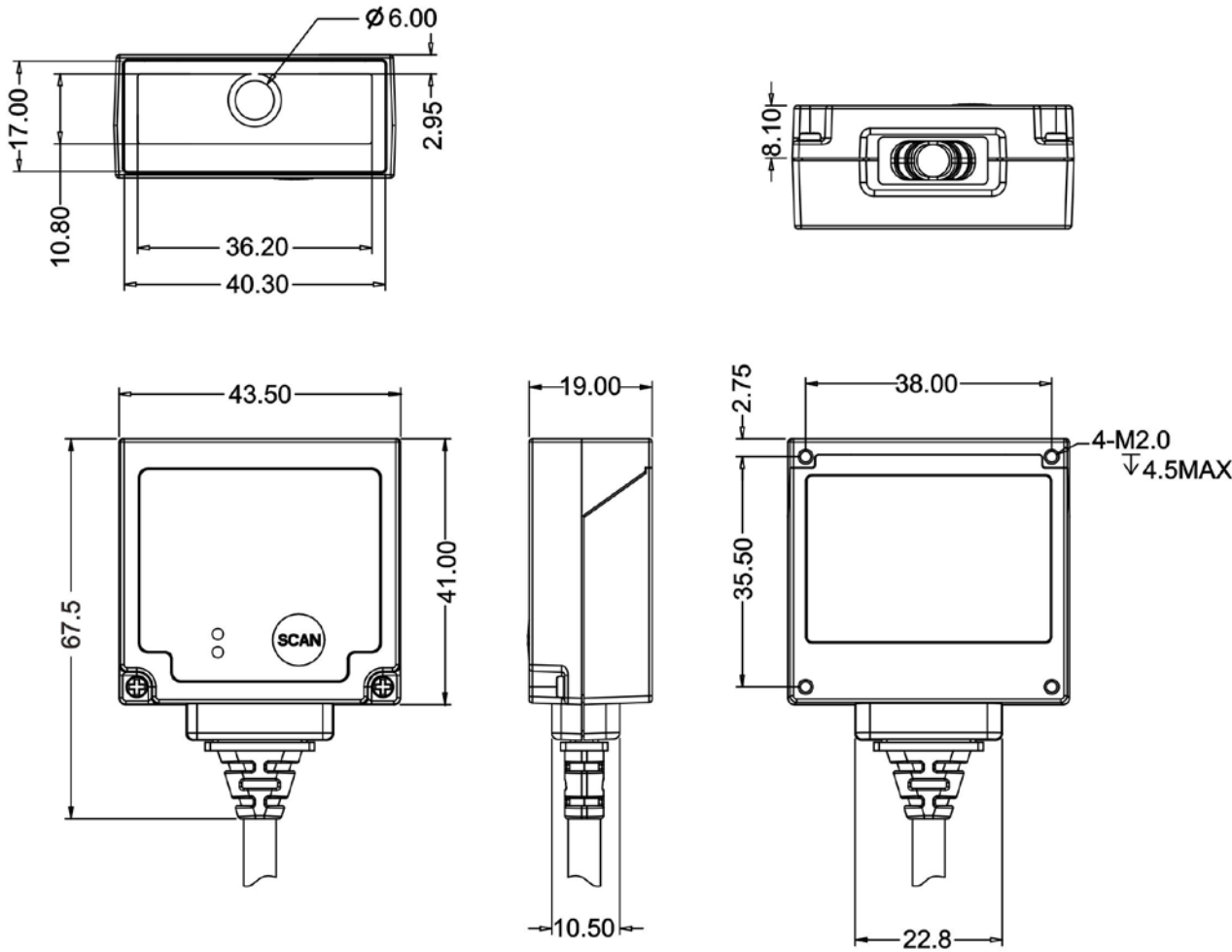
Figure 2-5 Mounting diagram
