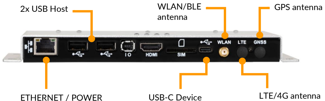
Picture 6 Rear panel of Nordic ID FR22 (communications)
