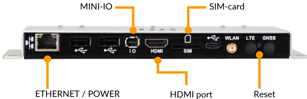
Picture 5 Rear panel of Nordic ID FR22 (operation)
