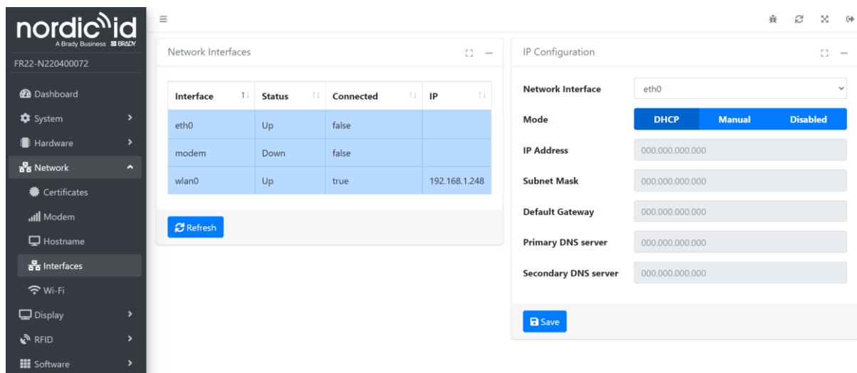
Screenshot 12 Network settings screen
