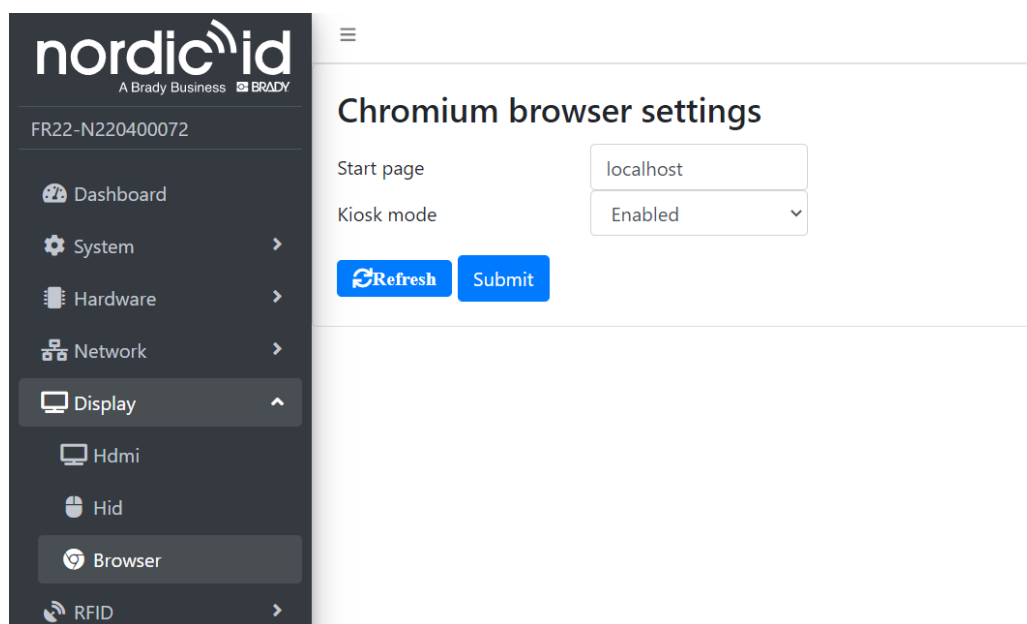
Screenshot 11 Chromium browser settings
