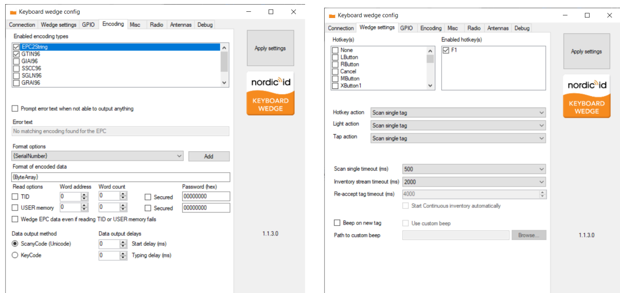
Screenshot 4 Nordic ID NUR Wedge for Microsoft Windows
