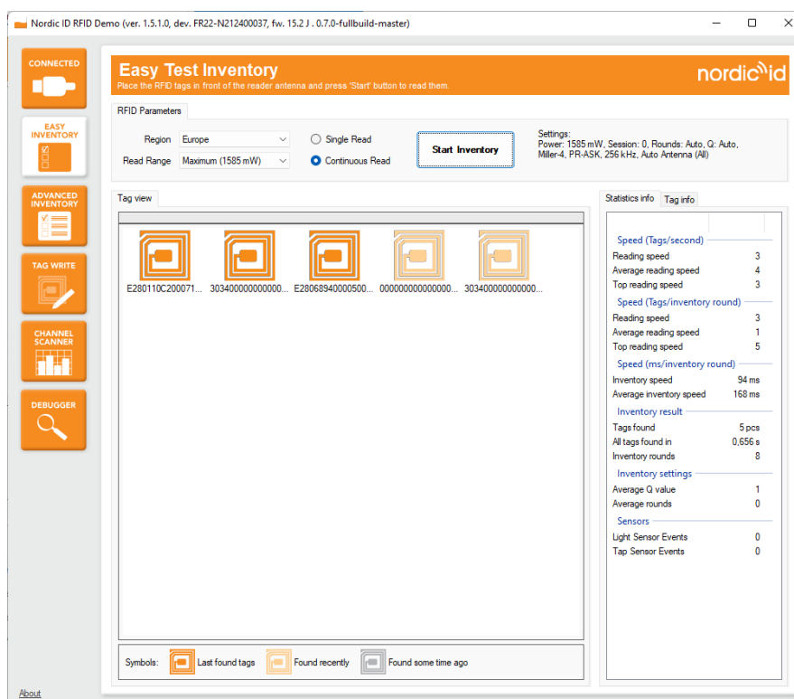
Screenshot 1 Nordic ID Demo for Microsoft Windows
