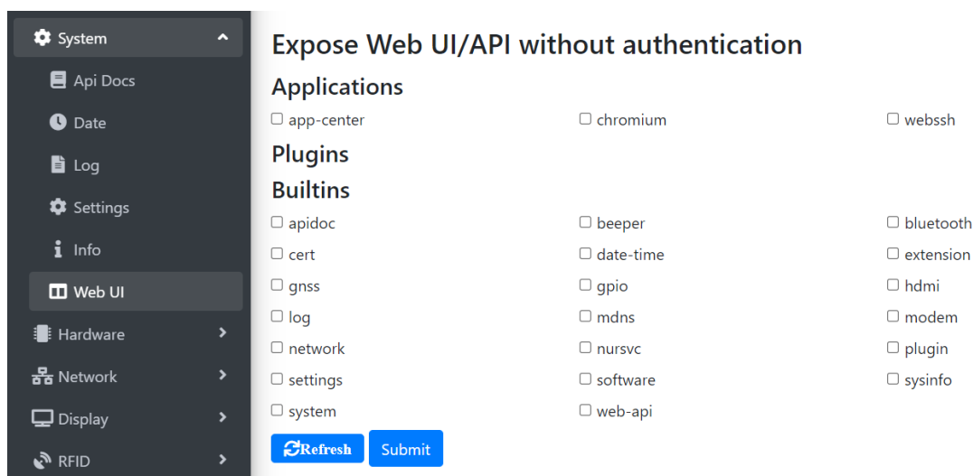
Screenshot 10 Web UI settings screen (2/2)
