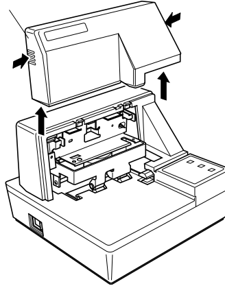
Printer cover
